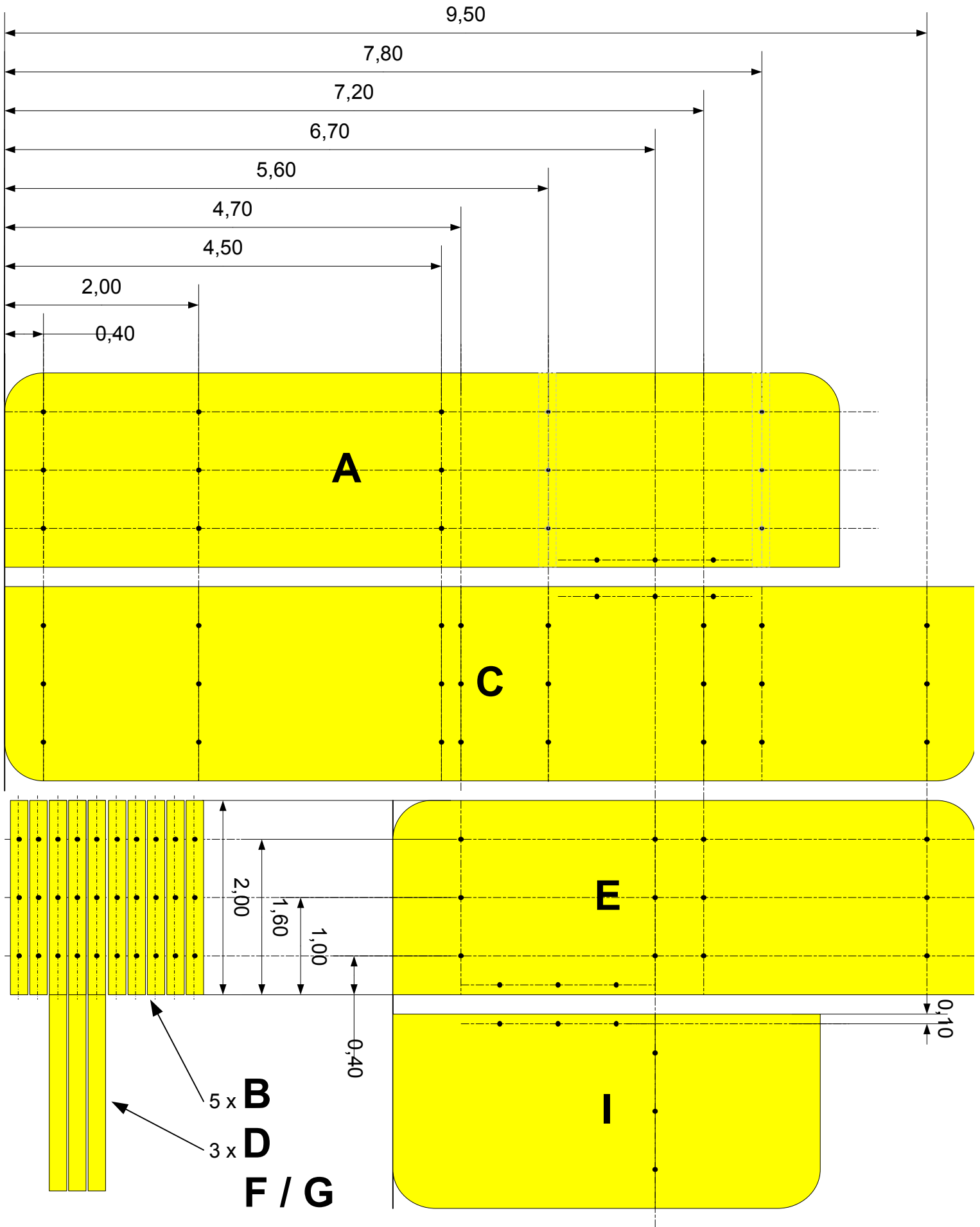
Eckregal 01 Bohrbild pm 08-02-14
